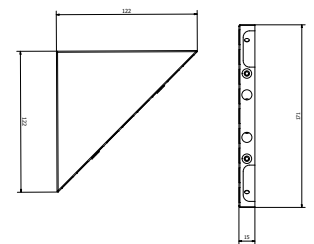
Corner Bracket
